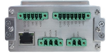
RS 485/232 + Ethernet (MODBUS RTU/TCP)
